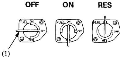
(1) Fuel valve
