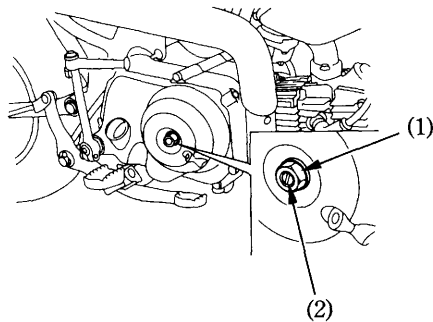
(2) Clutch adjuster
